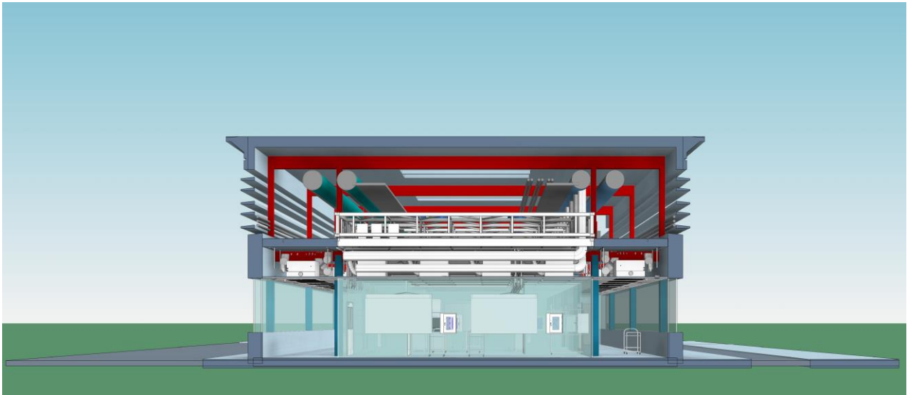
1 EXYTE_VACCINE PRODUCTION PLANT_CROSS SECTION
